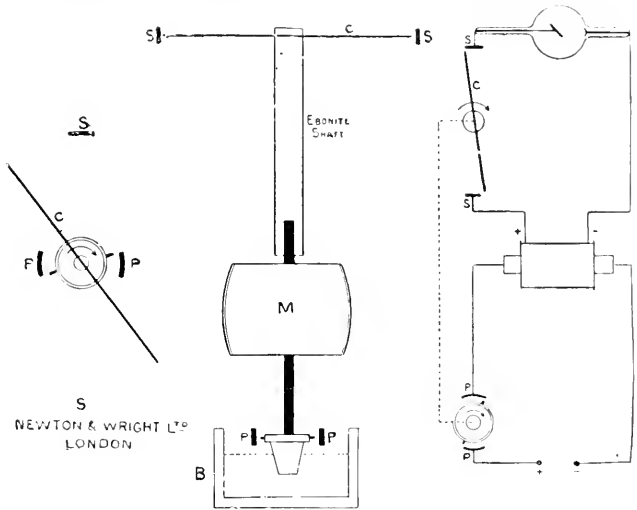
FIG. 193.—Diagram of connections for Morton rectifier.
